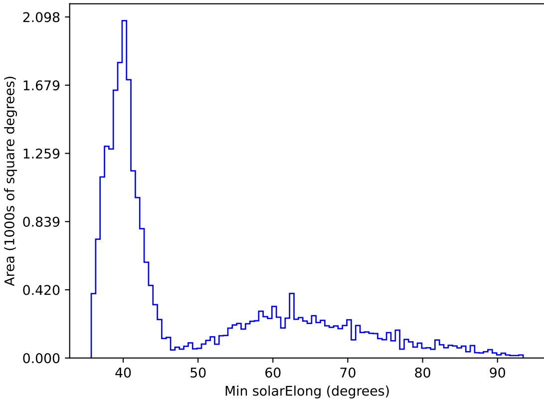
too_elab_r256_d2_gz_v3.4_10yrs All sky all bands: Min solarElong
