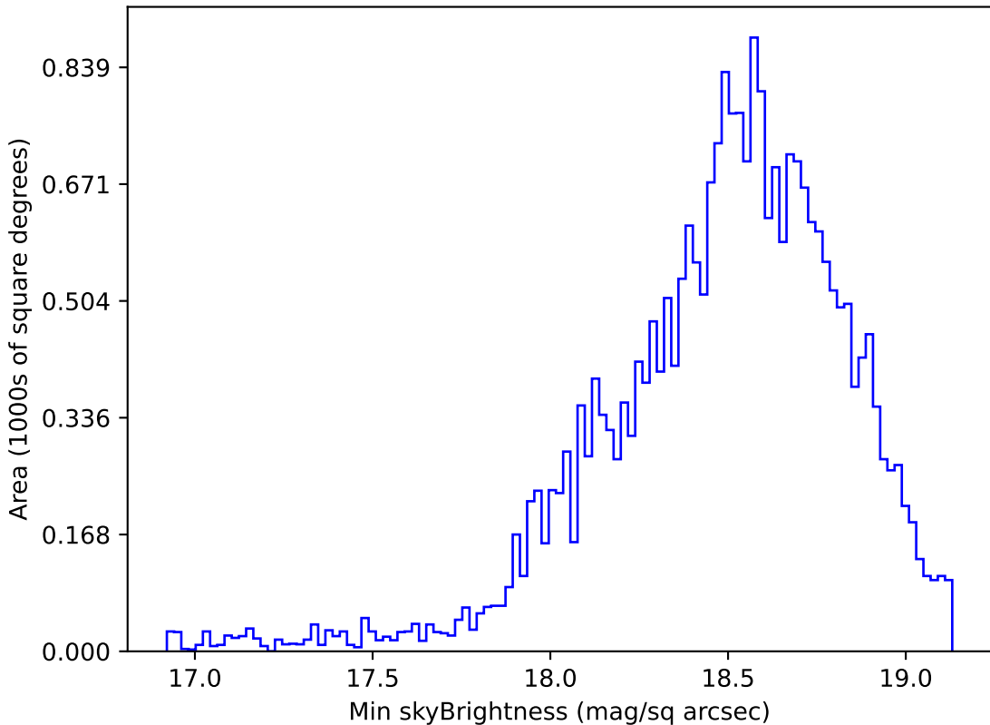
too_elab_r256_d2_gz_v3.4_10yrs Yr 1 z band: Min skyBrightness
