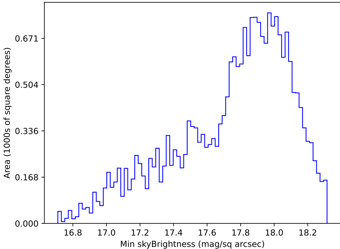
too_elab_r256_d2_gz_v3.4_10yrs Yr 1 y band: Min skyBrightness
