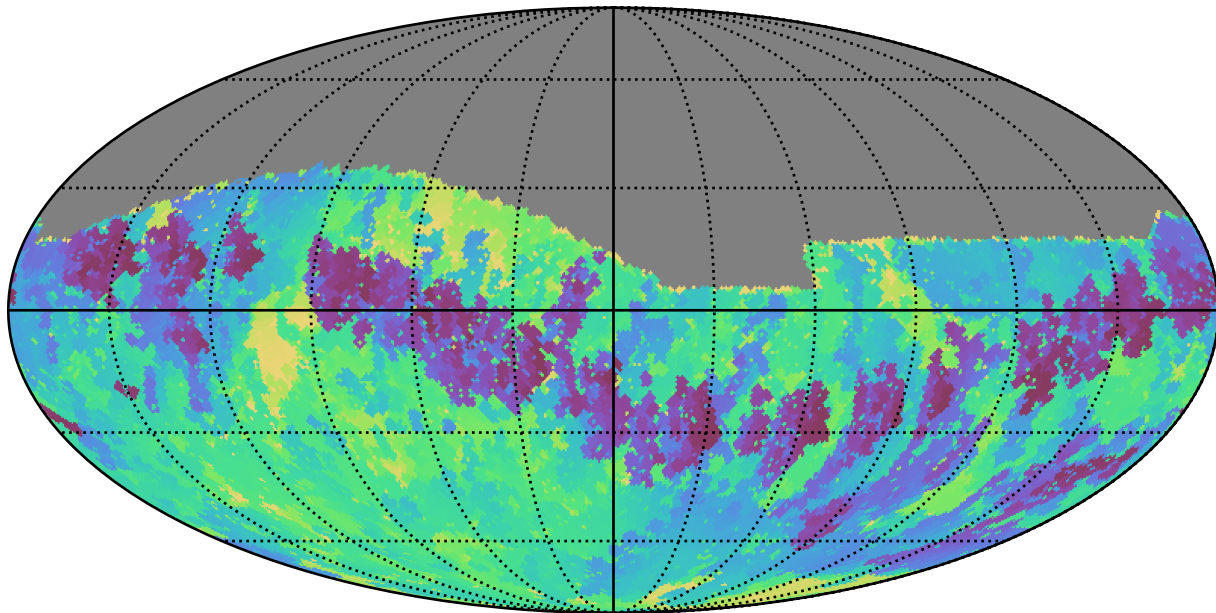
too_elab_r256_d2_gz_v3.4_10yrs Yr 1 i band: Min skyBrightness
