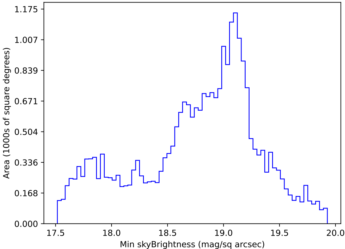
too_elab_r256_d2_gz_v3.4_10yrs Yr 1 i band: Min skyBrightness
