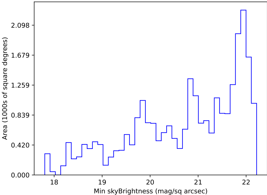
too_elab_r256_d2_gz_v3.4_10yrs Yr 1 g band: Min skyBrightness
