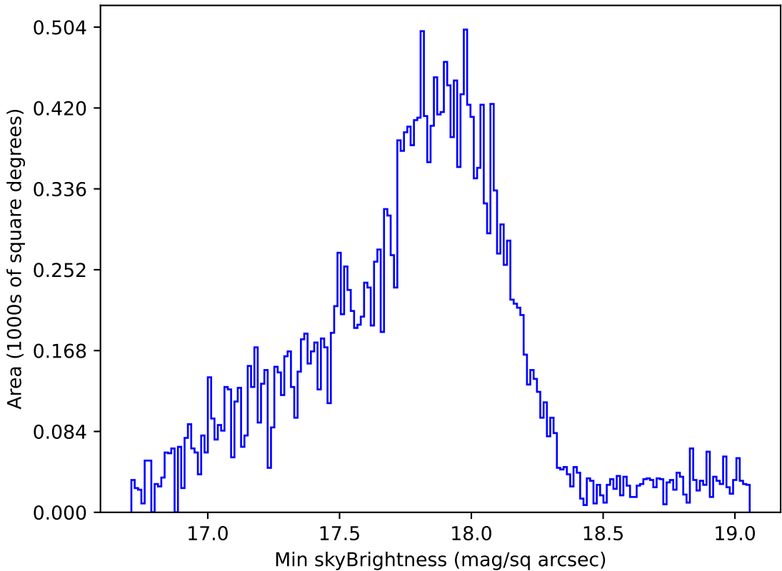
too_elab_r256_d2_gz_v3.4_10yrs Yr 1 all bands: Min skyBrightness
