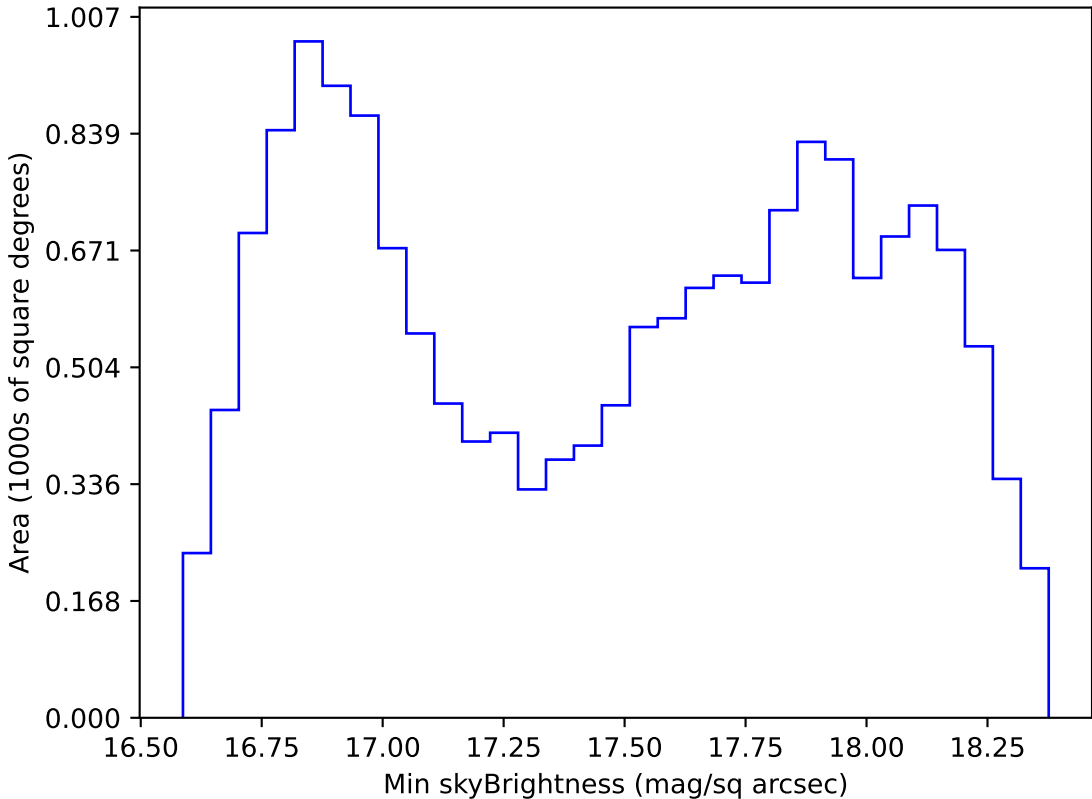
too_elab_r256_d2_gz_v3.4_10yrs WFD z band: Min skyBrightness
