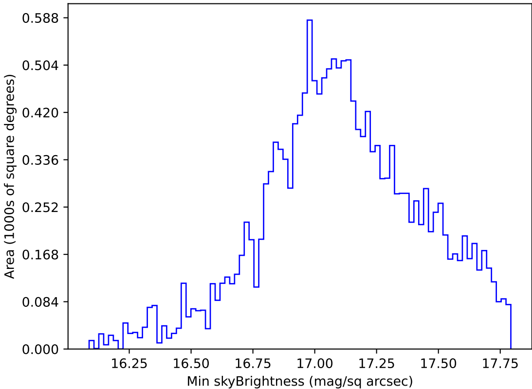
too_elab_r256_d2_gz_v3.4_10yrs WFD y band: Min skyBrightness
