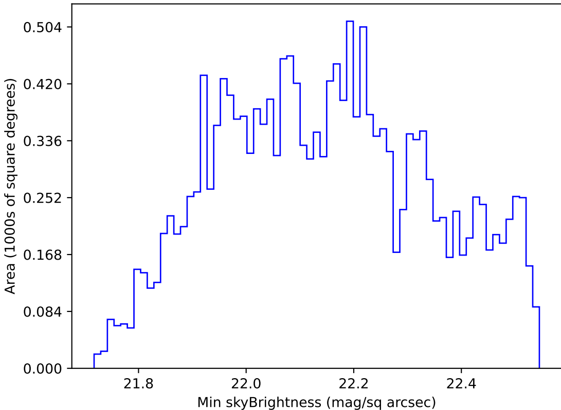
too_elab_r256_d2_gz_v3.4_10yrs WFD u band: Min skyBrightness
