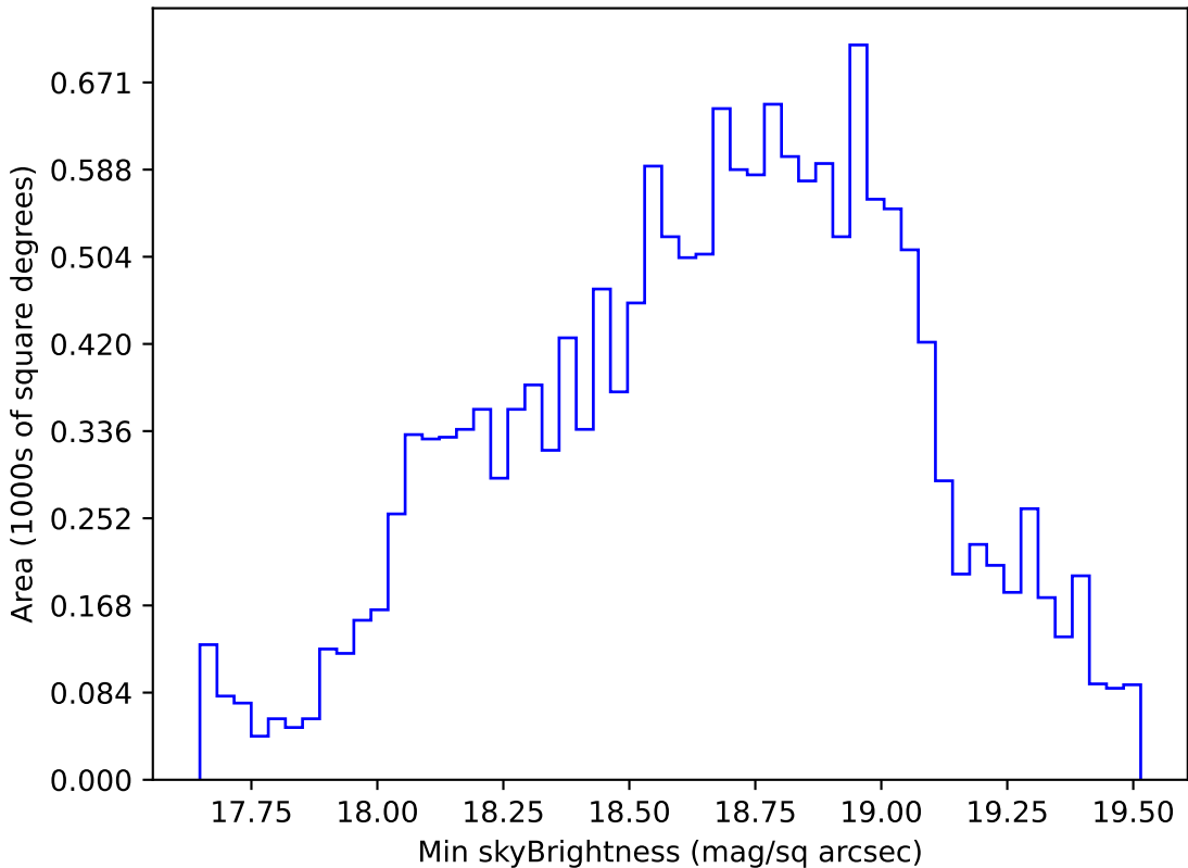
too_elab_r256_d2_gz_v3.4_10yrs WFD r band: Min skyBrightness
