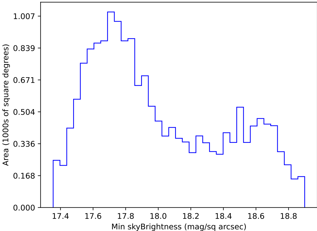
too_elab_r256_d2_gz_v3.4_10yrs WFD i band: Min skyBrightness
