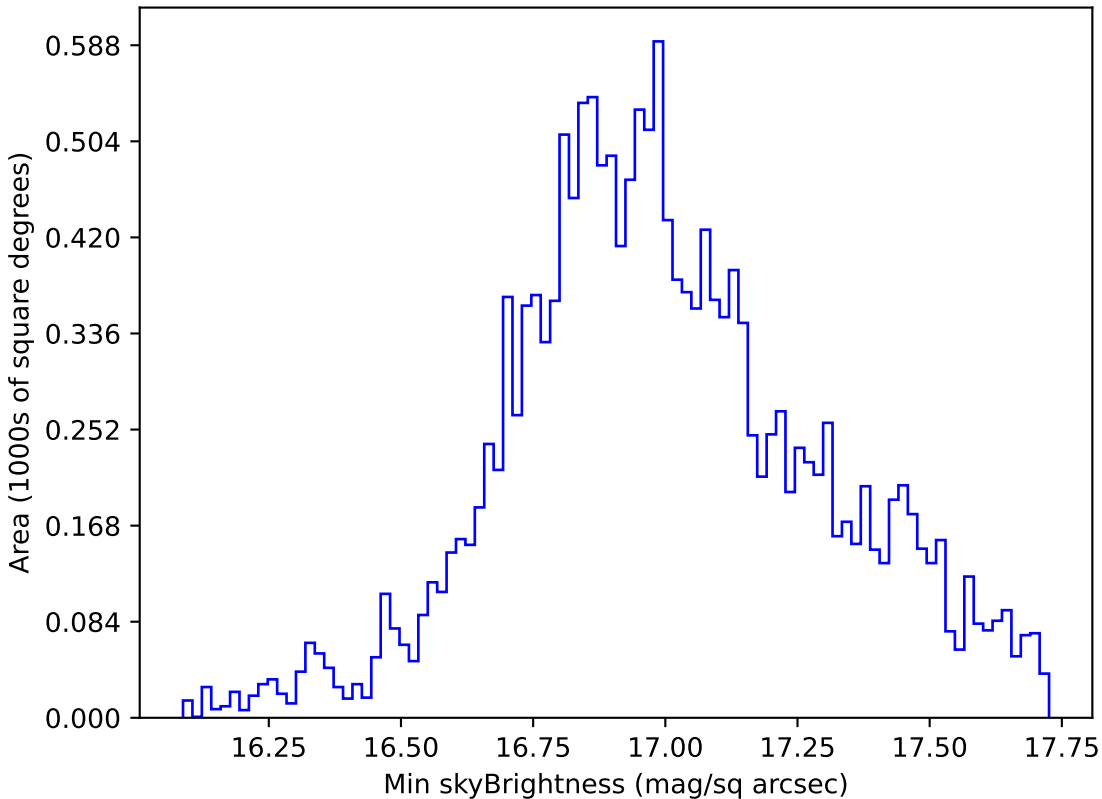
too_elab_r256_d2_gz_v3.4_10yrs WFD all bands: Min skyBrightness
