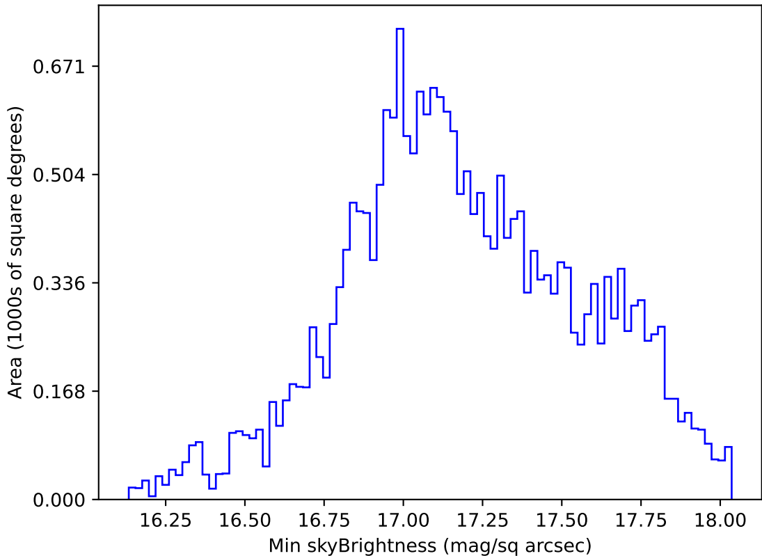
too_elab_r256_d2_gz_v3.4_10yrs All sky y band: Min skyBrightness
