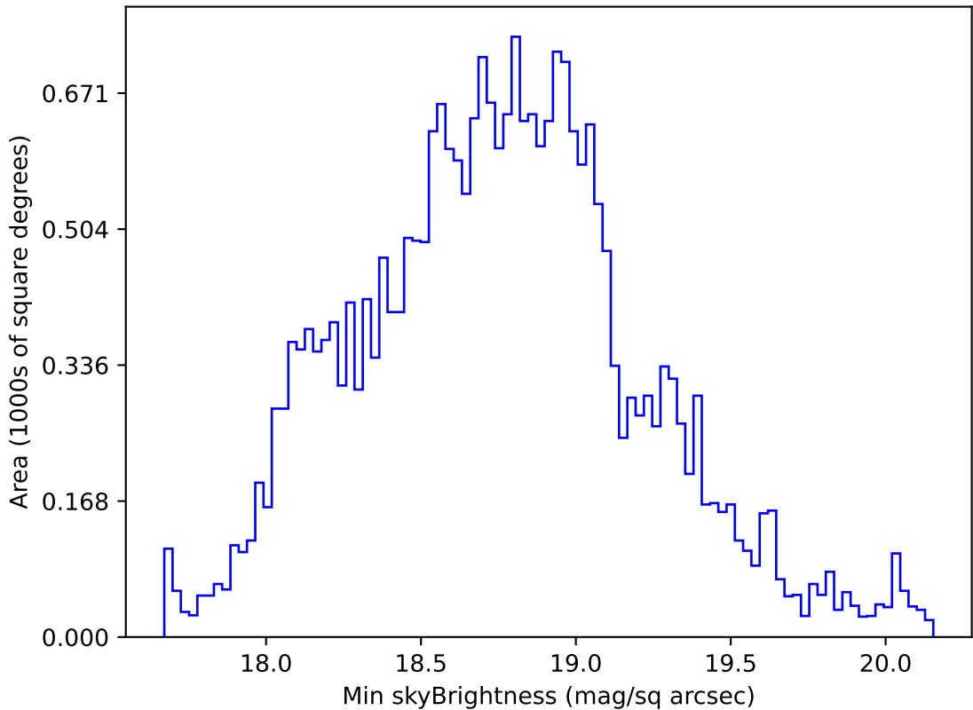
too_elab_r256_d2_gz_v3.4_10yrs All sky r band: Min skyBrightness
