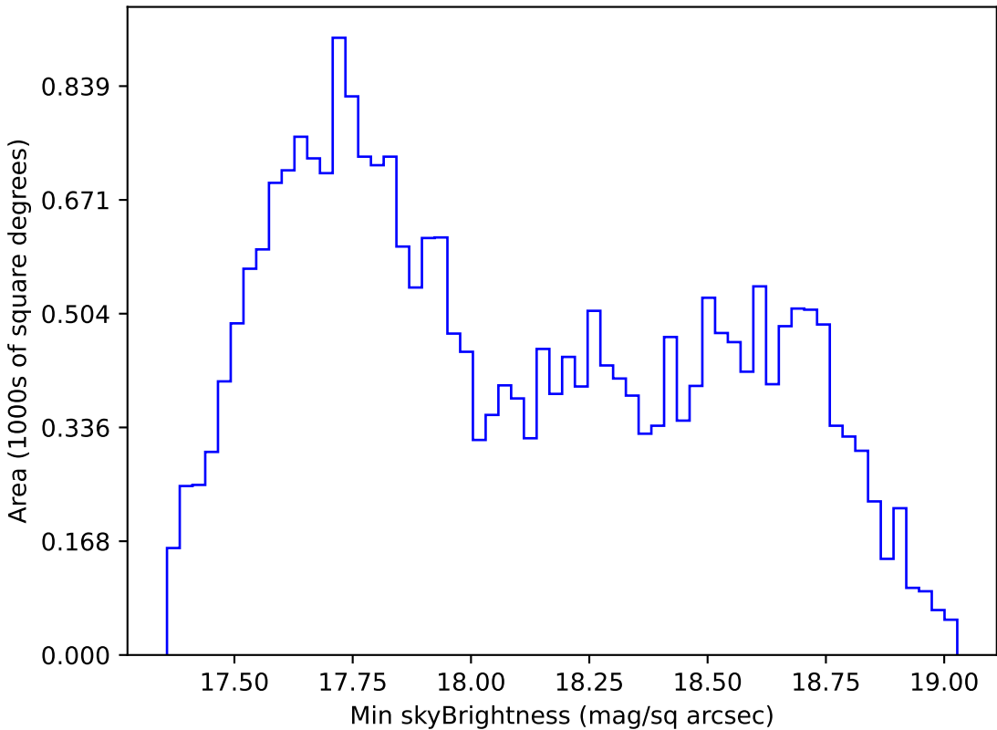
too_elab_r256_d2_gz_v3.4_10yrs All sky i band: Min skyBrightness
