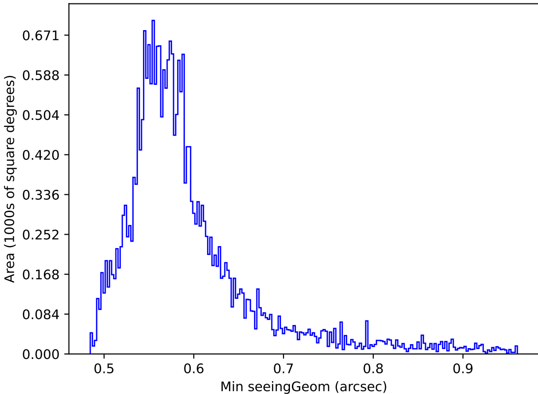
too_elab_r256_d2_gz_v3.4_10yrs Yr 1 all bands: Min seeingGeom
