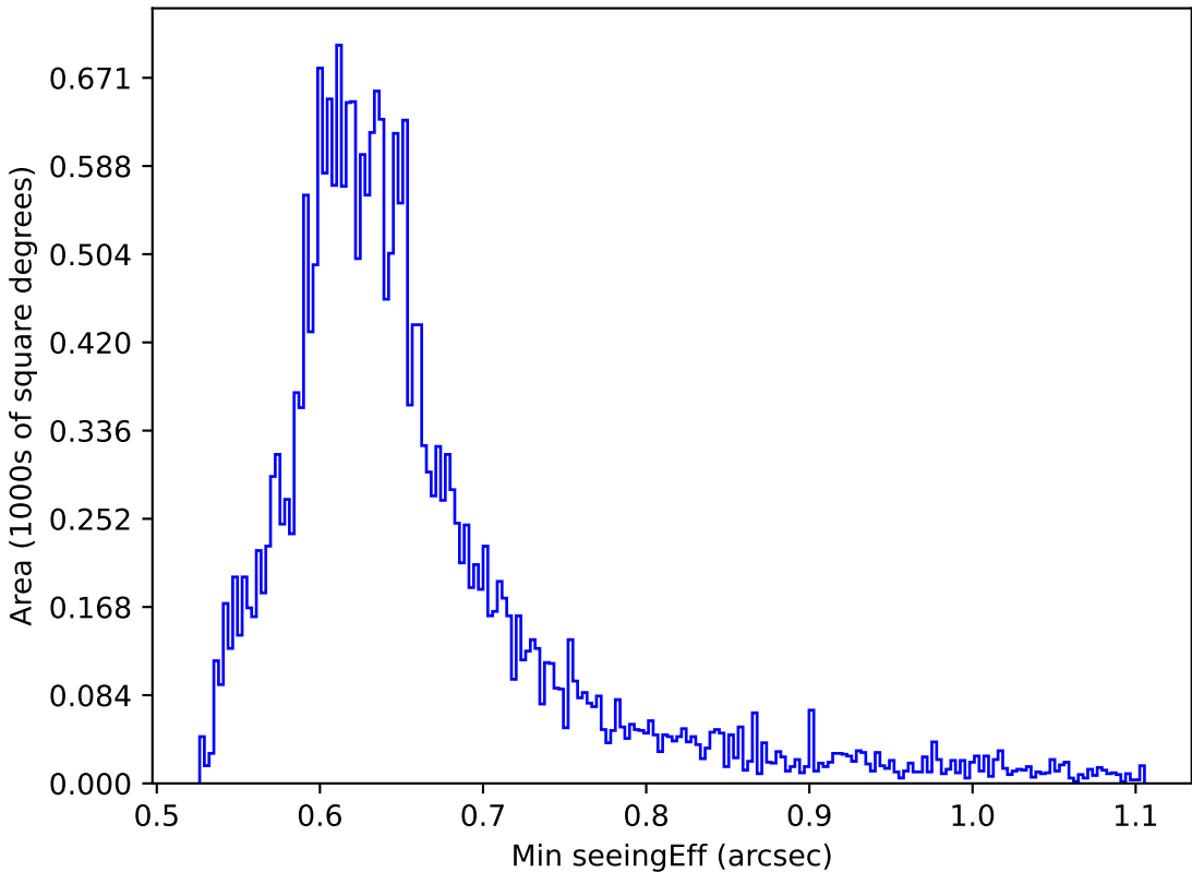
too_elab_r256_d2_gz_v3.4_10yrs Yr 1 all bands: Min seeingEff
