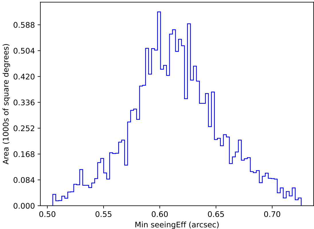
too_elab_r256_d2_gz_v3.4_10yrs WFD z band: Min seeingEff
