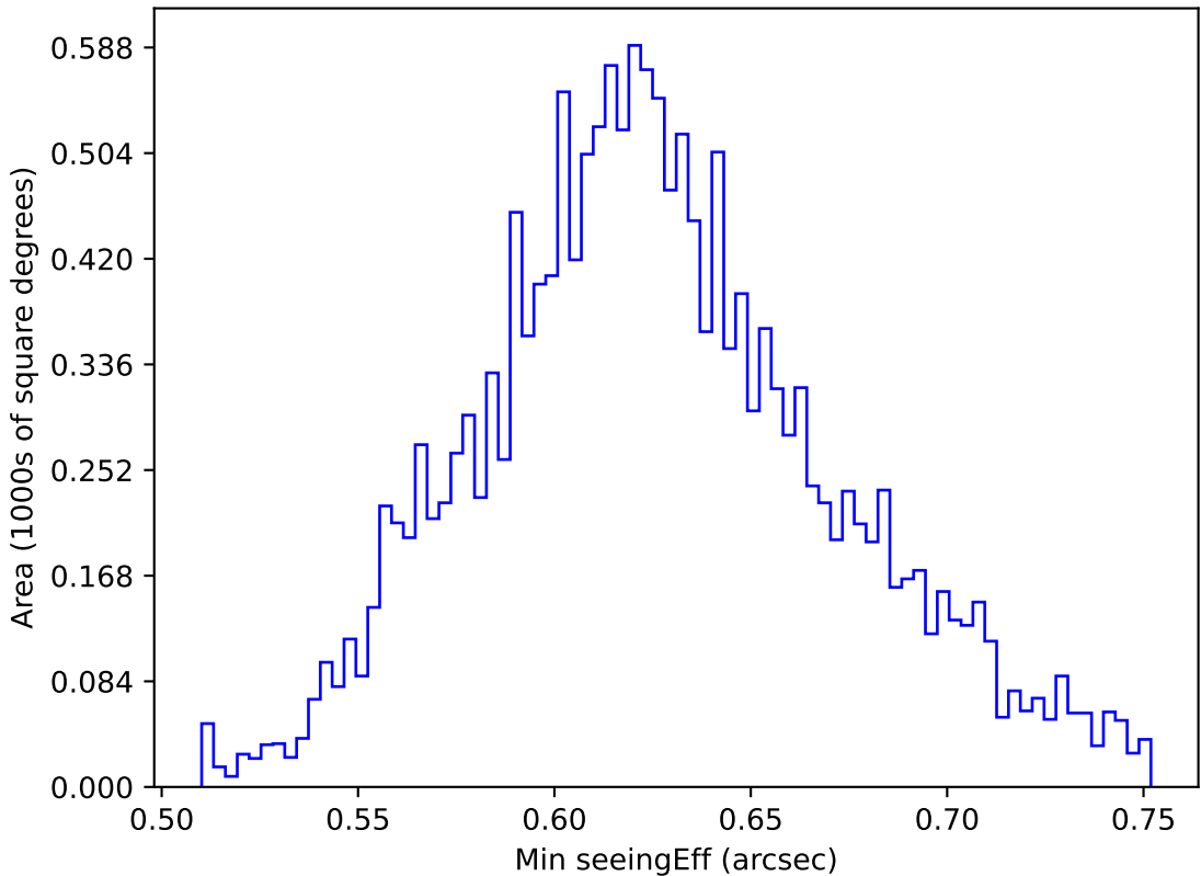
too_elab_r256_d2_gz_v3.4_10yrs WFD y band: Min seeingEff
