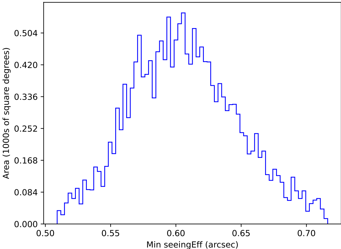
too_elab_r256_d2_gz_v3.4_10yrs WFD i band: Min seeingEff
