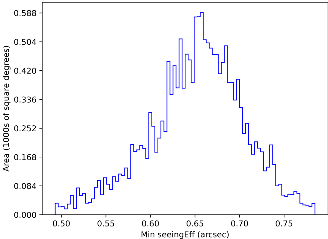
too_elab_r256_d2_gz_v3.4_10yrs WFD g band: Min seeingEff
