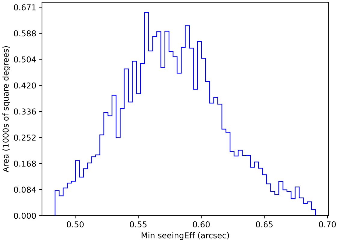
too_elab_r256_d2_gz_v3.4_10yrs WFD all bands: Min seeingEff
