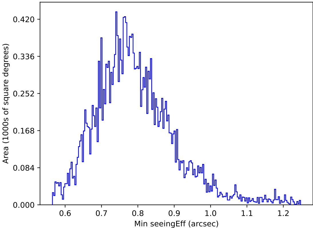
too_elab_r256_d2_gz_v3.4_10yrs All sky u band: Min seeingEff
