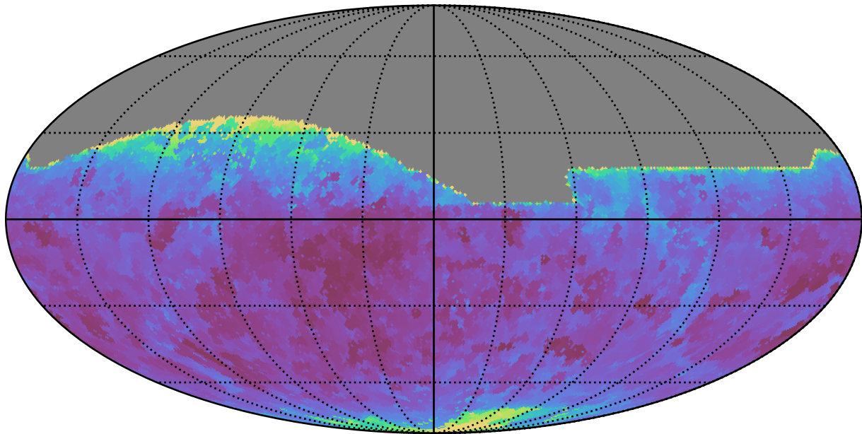
too_elab_r256_d2_gz_v3.4_10yrs All sky r band: Min seeingEff
