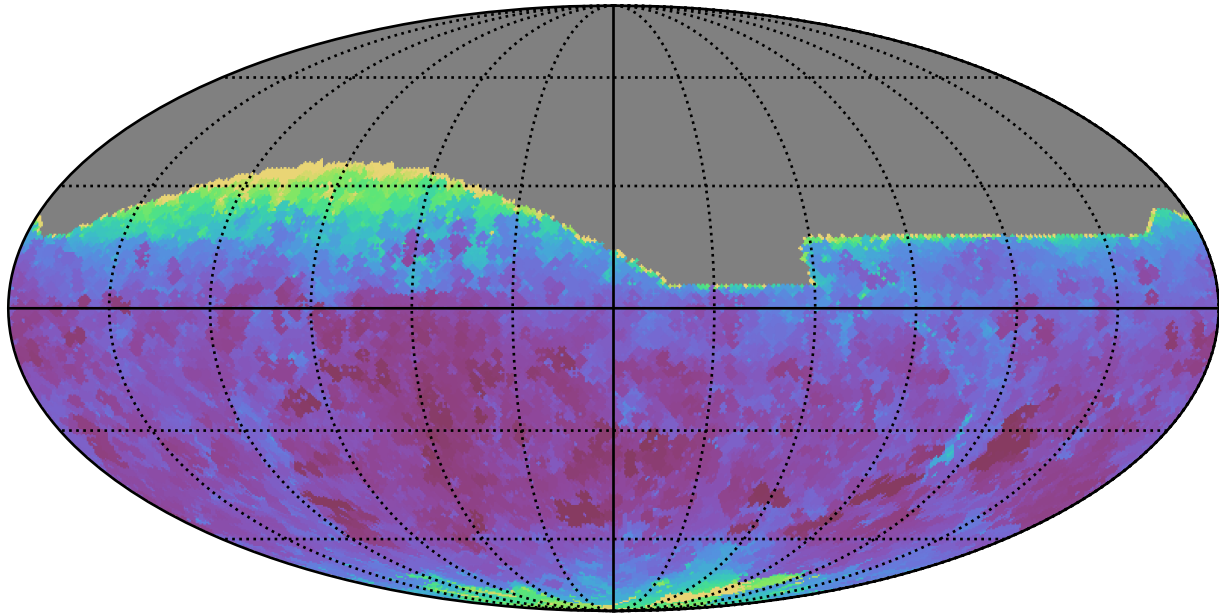
too_elab_r256_d2_gz_v3.4_10yrs All sky i band: Min seeingEff
