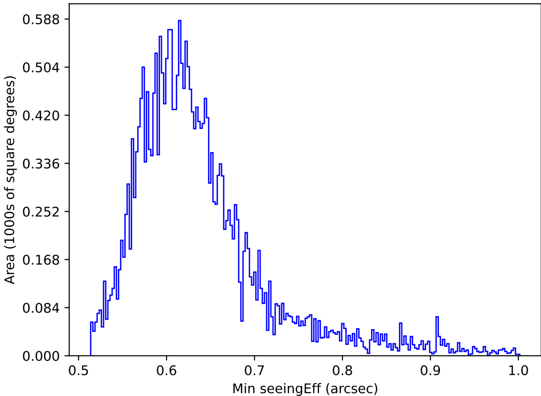
too_elab_r256_d2_gz_v3.4_10yrs All sky i band: Min seeingEff
