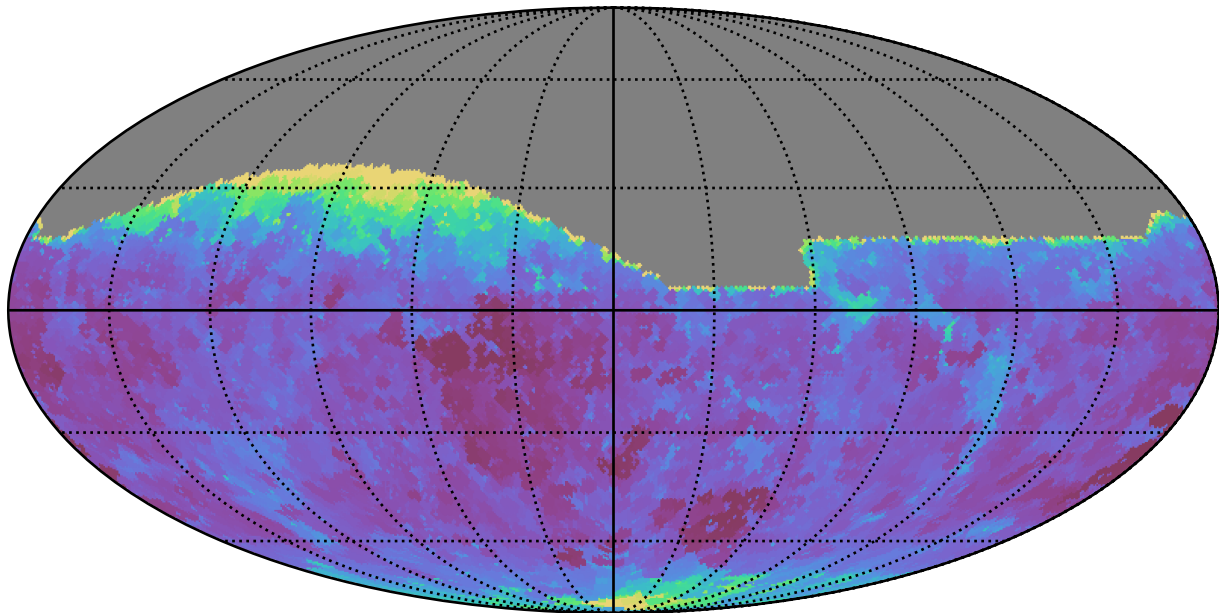
too_elab_r256_d2_gz_v3.4_10yrs All sky g band: Min seeingEff
