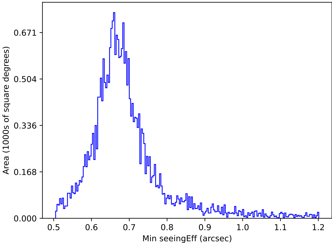
too_elab_r256_d2_gz_v3.4_10yrs All sky g band: Min seeingEff
