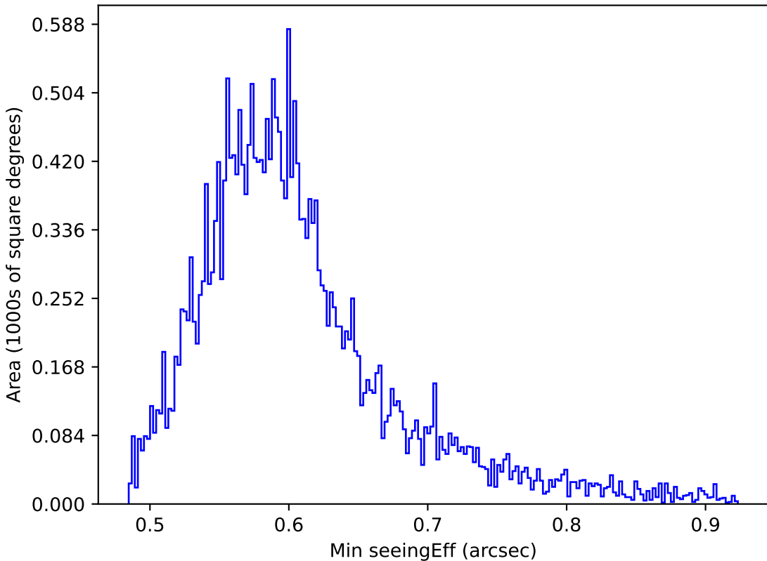
too_elab_r256_d2_gz_v3.4_10yrs All sky all bands: Min seeingEff
