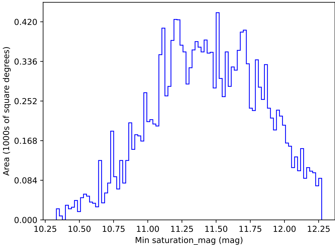
too_elab_r256_d2_gz_v3.4_10yrs WFD u band: Min saturation_mag
