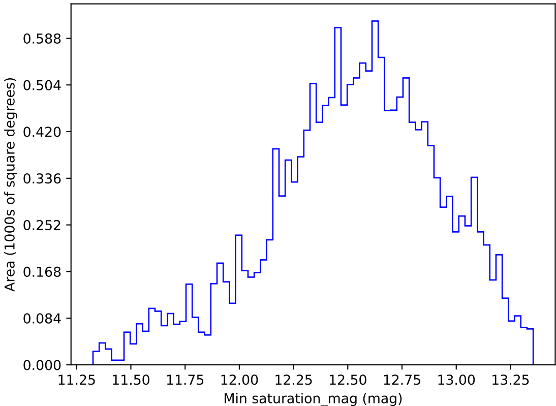
too_elab_r256_d2_gz_v3.4_10yrs WFD r band: Min saturation_mag
