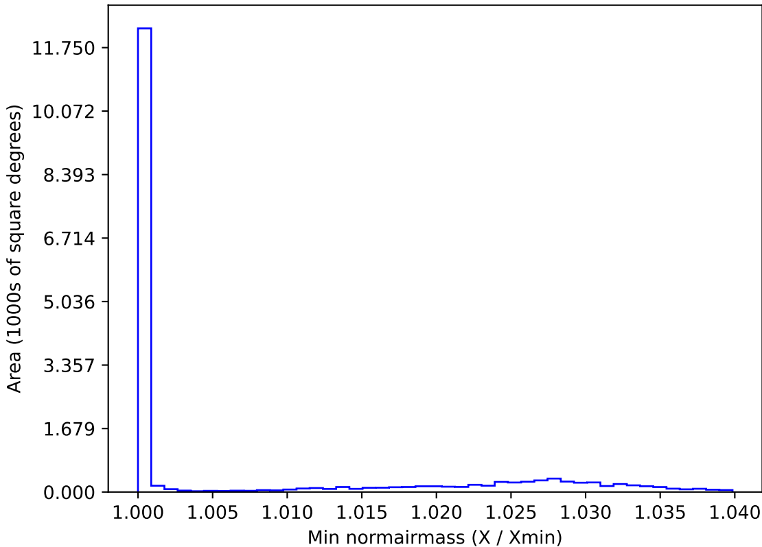
too_elab_r256_d2_gz_v3.4_10yrs WFD y band: Min normairmass
