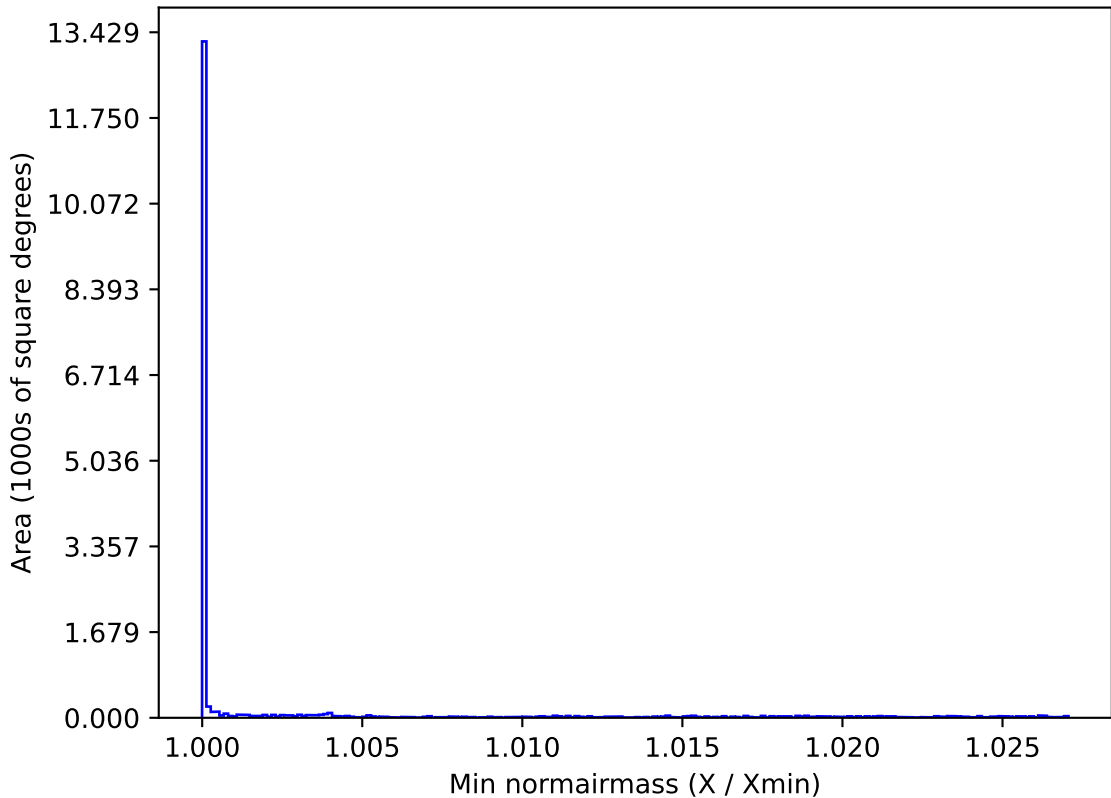
too_elab_r256_d2_gz_v3.4_10yrs WFD all bands: Min normairmass
