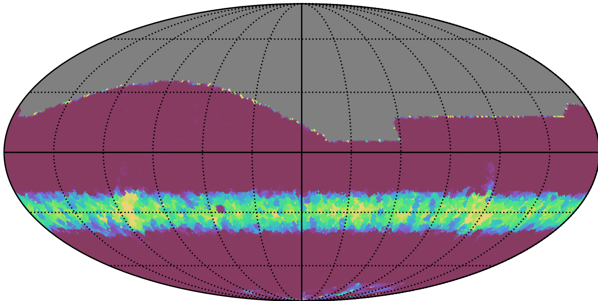
too_elab_r256_d2_gz_v3.4_10yrs All sky r band: Min normairmass
