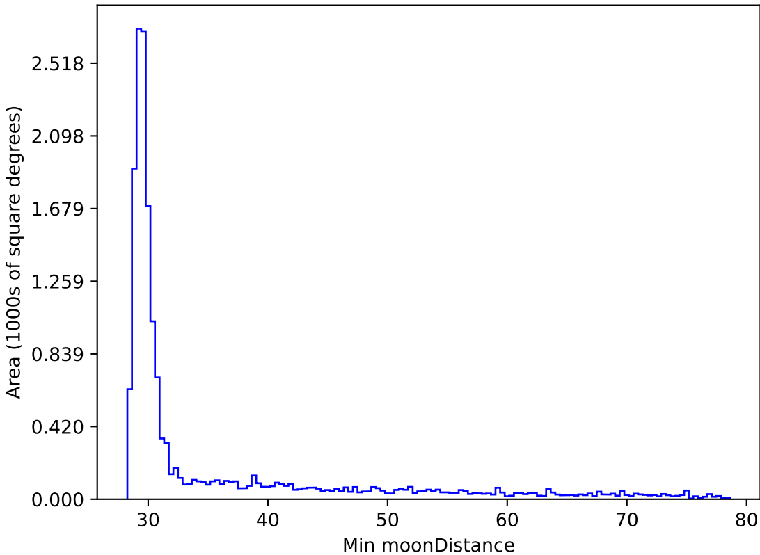
too_elab_r256_d2_gz_v3.4_10yrs WFD y band: Min moonDistance
