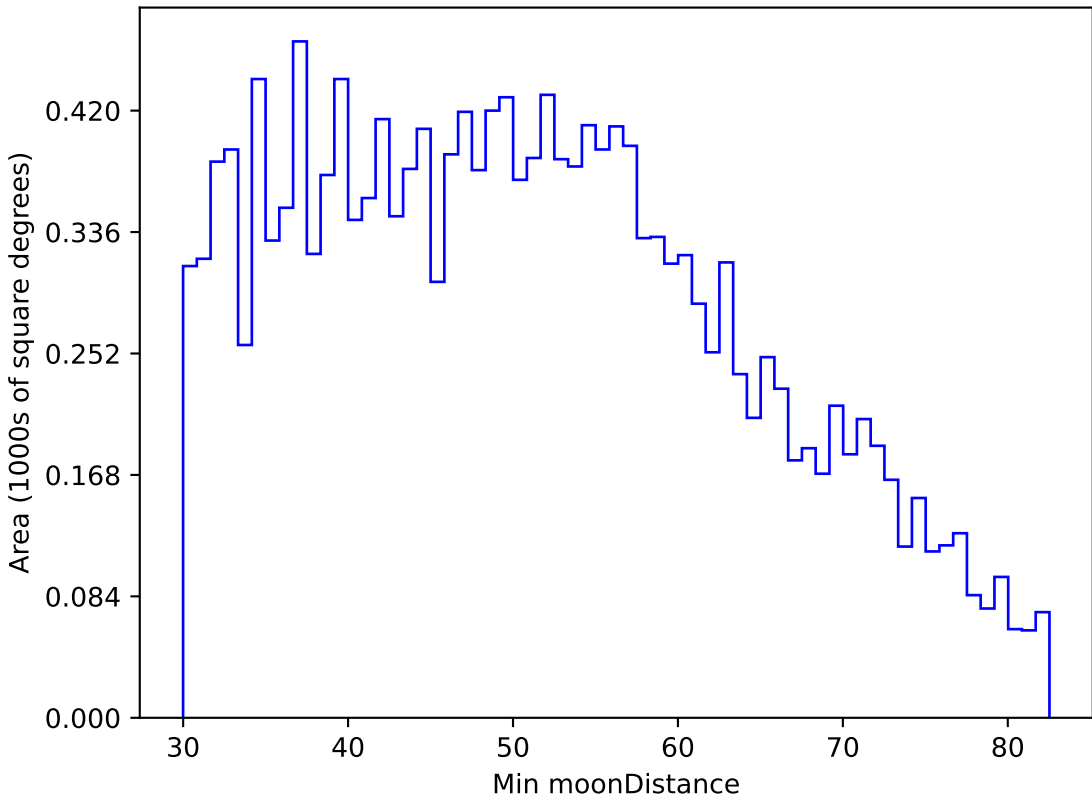
too_elab_r256_d2_gz_v3.4_10yrs WFD u band: Min moonDistance
