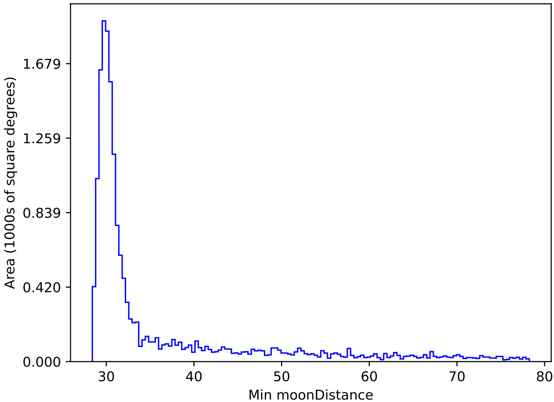
too_elab_r256_d2_gz_v3.4_10yrs WFD i band: Min moonDistance
