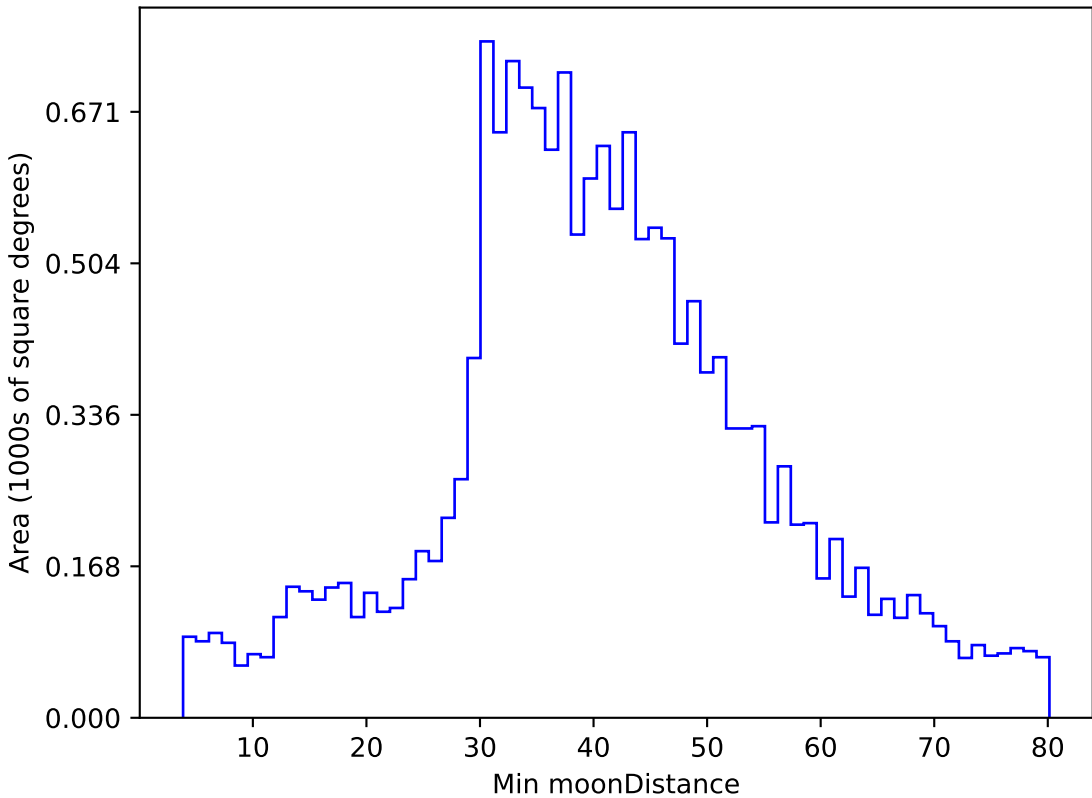
too_elab_r256_d2_gz_v3.4_10yrs WFD g band: Min moonDistance
