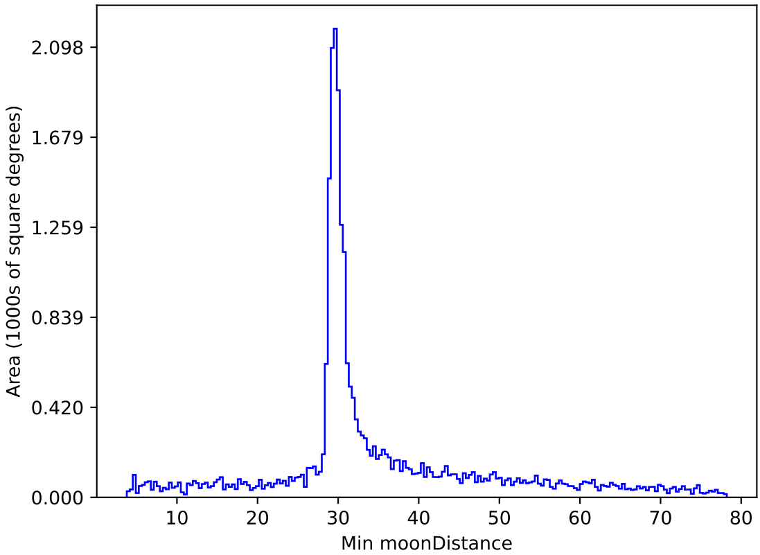
too_elab_r256_d2_gz_v3.4_10yrs All sky z band: Min moonDistance
