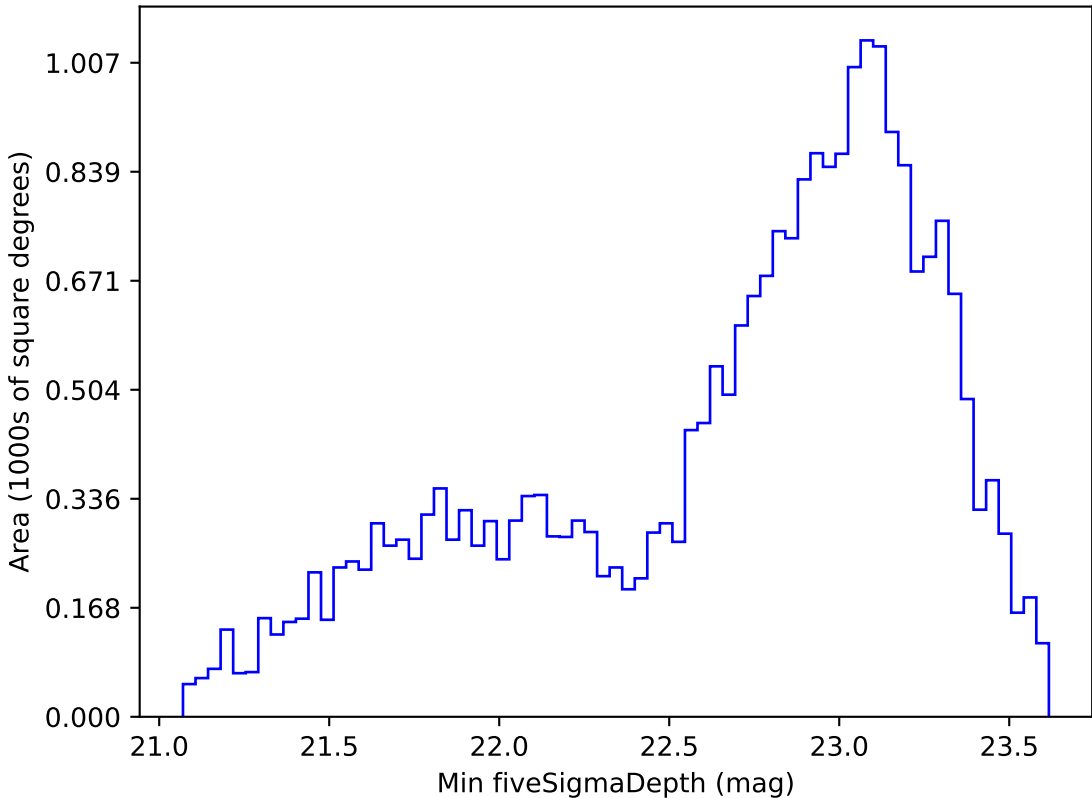
too_elab_r256_d2_gz_v3.4_10yrs Yr 1 i band: Min fiveSigmaDepth
