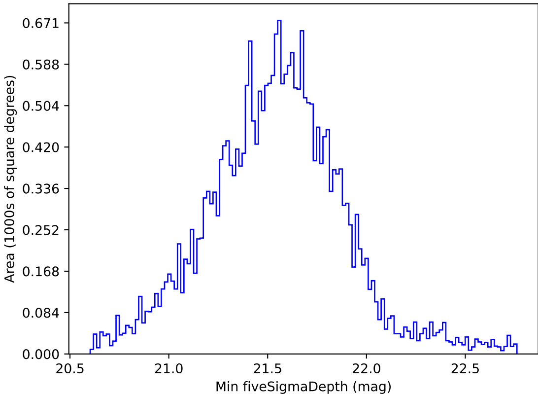
too_elab_r256_d2_gz_v3.4_10yrs Yr 1 all bands: Min fiveSigmaDepth
