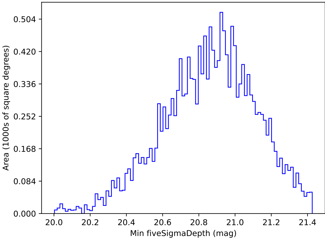
too_elab_r256_d2_gz_v3.4_10yrs WFD y band: Min fiveSigmaDepth
