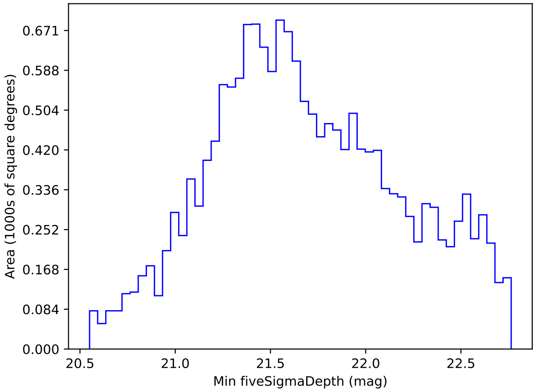
too_elab_r256_d2_gz_v3.4_10yrs WFD i band: Min fiveSigmaDepth
