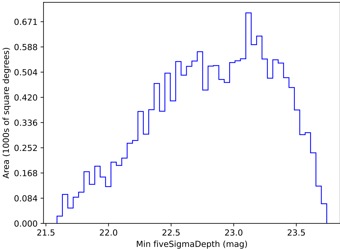
too_elab_r256_d2_gz_v3.4_10yrs WFD g band: Min fiveSigmaDepth
