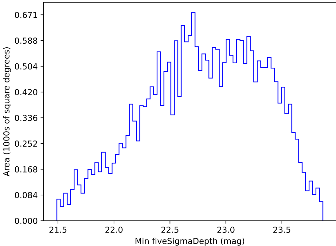
too_elab_r256_d2_gz_v3.4_10yrs All sky g band: Min fiveSigmaDepth
