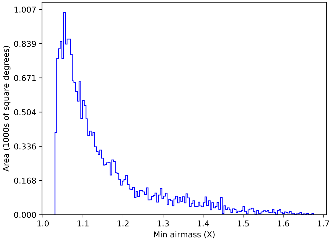
too_elab_r256_d2_gz_v3.4_10yrs Yr 1 u band: Min airmass
