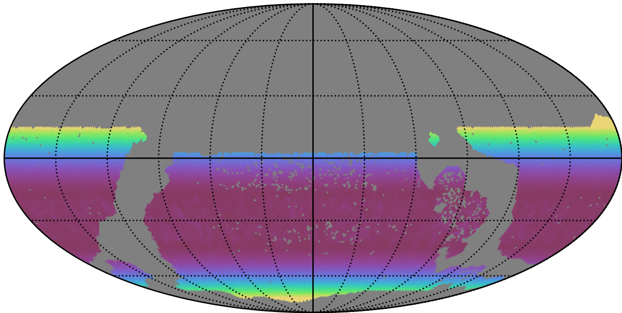
too_elab_r256_d2_gz_v3.4_10yrs WFD y band: Min airmass
