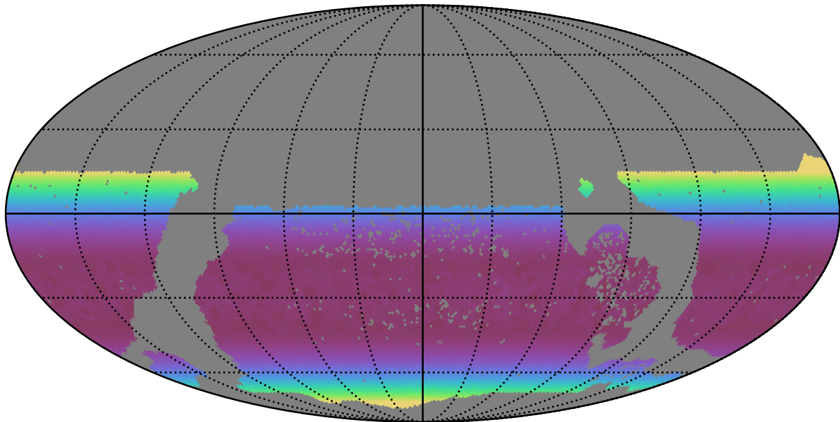
too_elab_r256_d2_gz_v3.4_10yrs WFD r band: Min airmass
