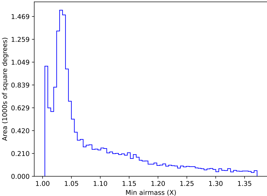
too_elab_r256_d2_gz_v3.4_10yrs WFD g band: Min airmass
